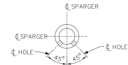
SECTION D-D HOLE ORIENTATION (TYP ALL SPARGERS) (DRAIN HOLES NOT SHOWN)
