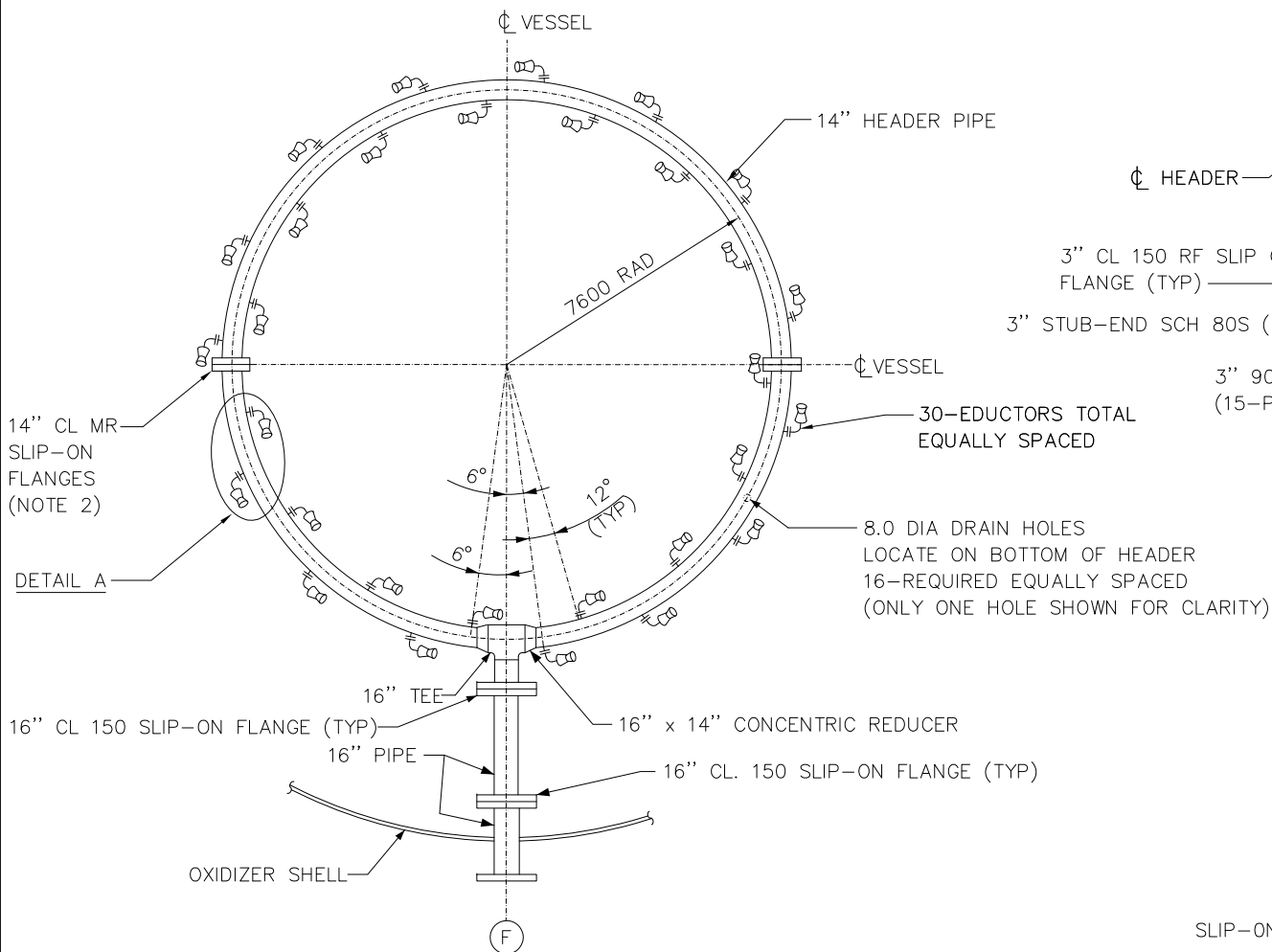
FEED/CIRCULATION DISTRIBUTOR
