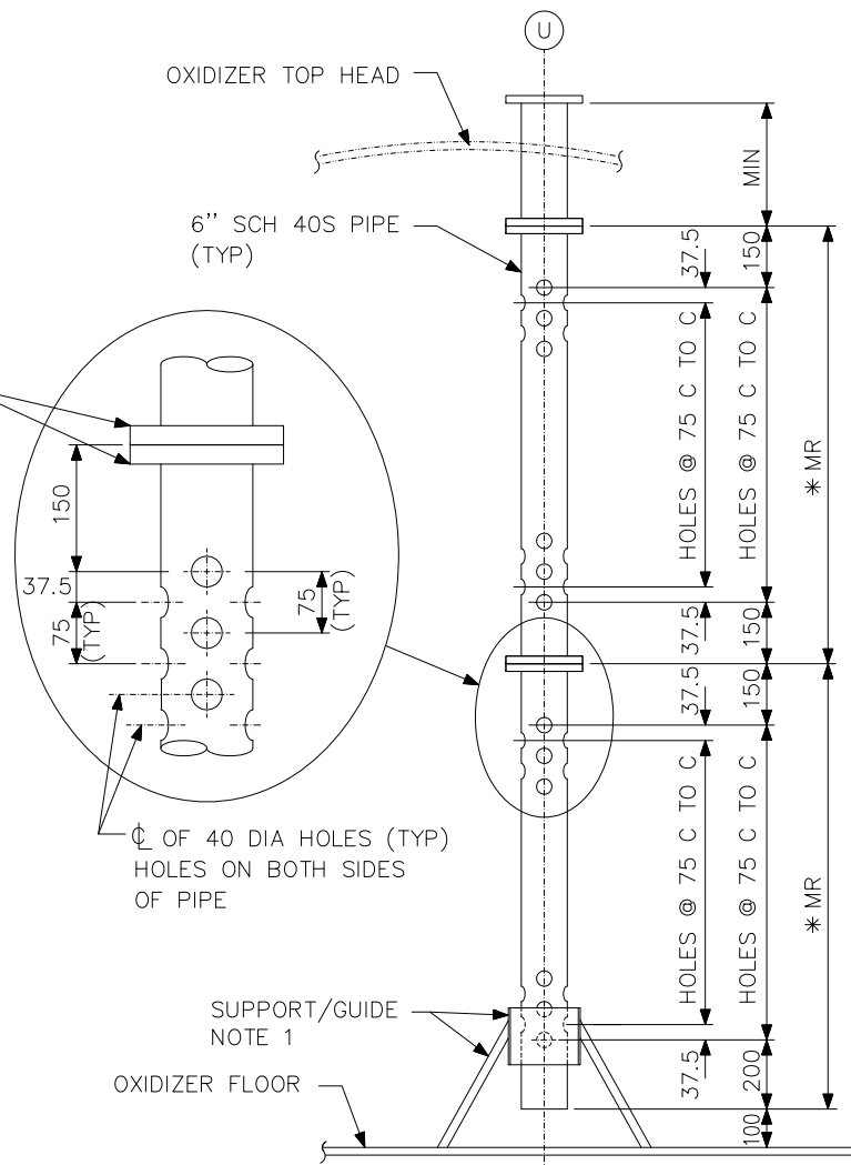
PIPE STILLING WELL
