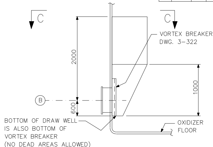
DETAIL B
