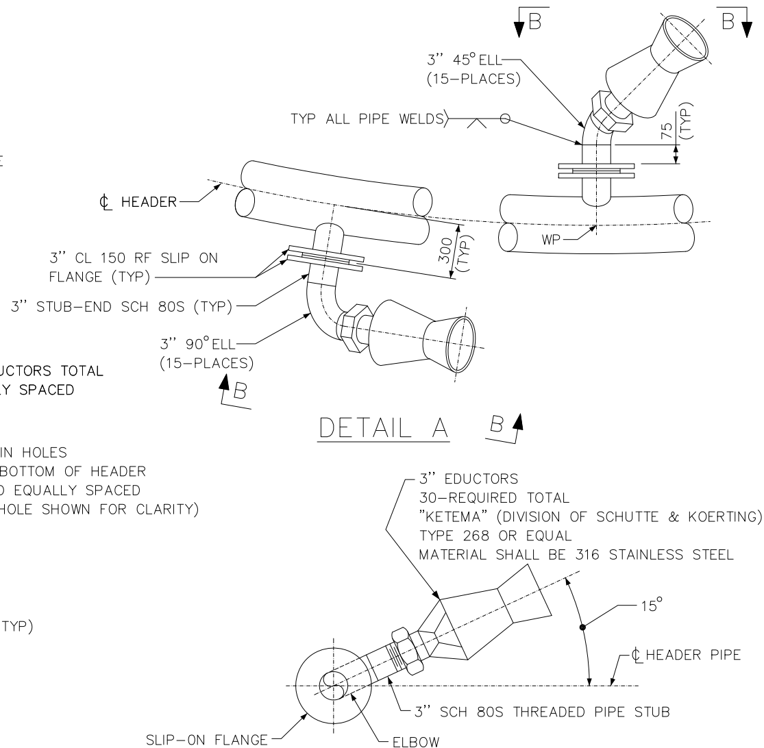
FINAL POSITIONING OF EDUCATORS SHALL BE DONE DURING INSTALLATION AT SITE (TYP FOR ALL EDUCATORS)
