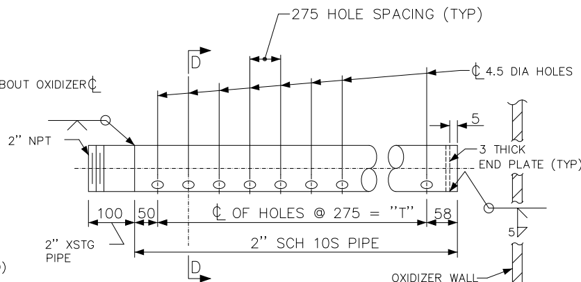
DETAIL C
